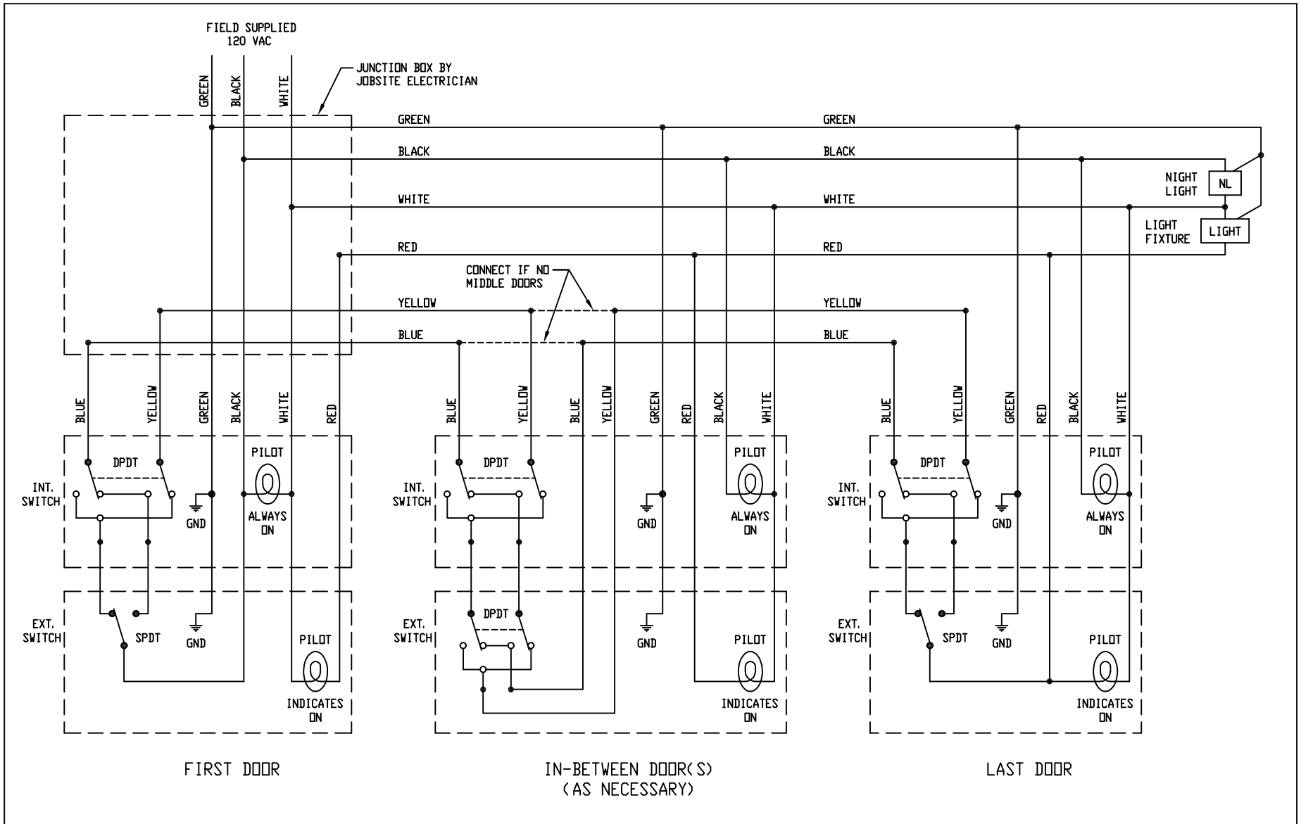
MULTIPLE ENTRANCE LIGHT CONTROL WIRING DIAGRAM
