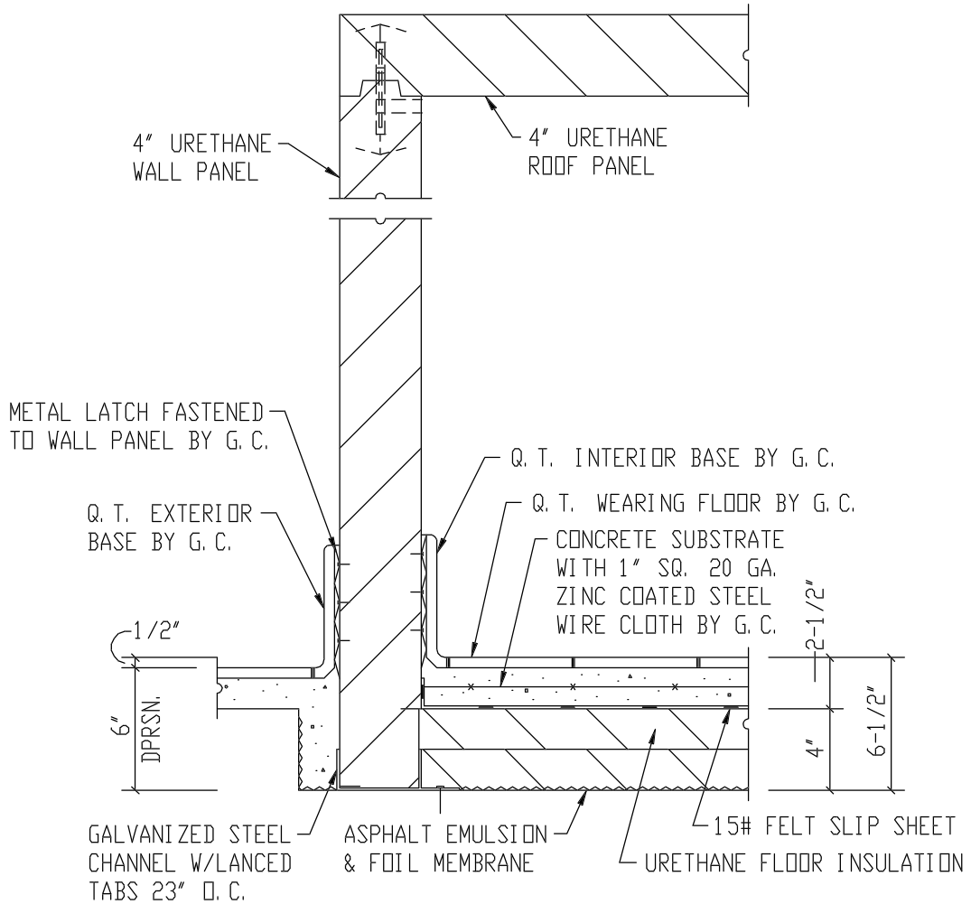
SECTION (@ WALL) 1-1/2" = 1'-0" (FD)
